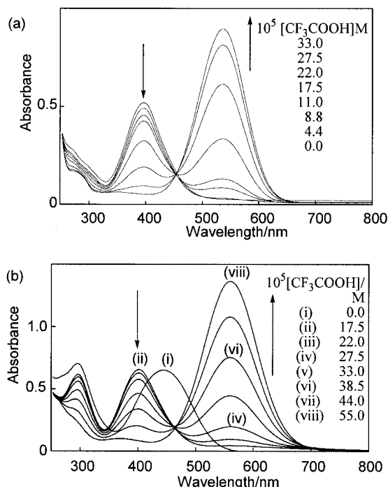
Figure 4. Change in the absorption spectra of (a) 1 ( 2.5 \times 10^{-5} M in \text{CHCl}_3 ) and (b) 4 ( 2.5 \times 10^{-5} M in \text{CHCl}_3 ) upon addition of \text{CF}_3\text{COOH}
