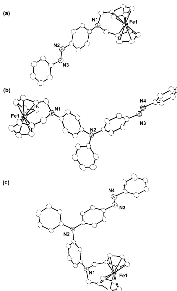
Figure 1. (a) An ORTEP drawing of 1 ; selected bond lengths (Å) and angles (°): C1–C11 1.497(9), C6–C12 1.500(9), N1–C11 1.467(7), N1–C12 1.484(8), N1–C13 1.355(8), N2–C16 1.402(8), N2–C19 1.436(8), N2–N3 1.276(7); C11–N1–C12 112.9(5), C11–N1–C13 122.9(5), C12–N1–C13 121.8(6), N1–C11–C1 114.5(5), N1–C12–C6 114.4(5), N2–C16–C15 116.9(6), N2–C16–C17 125.0(6), N2–N3–C19 113.3(6), N3–N2–C16 116.2(6), N3–C19–C20 123.8(7), N3–C19–C24 115.6(7); (b) An ORTEP drawing of 4 ; only one of the crystallographically independent molecules is shown; selected bond lengths (Å) and angles (°): C1–C11 1.52(1), C6–C12 1.51(1), N1–C11 1.44(1), N1–C12 1.46(1), N1–C13 1.393(8), N2–C16 1.433(8), N2–C19 1.410(8), N2–C25 1.429(8), N3–C28 1.456(8), N4–C31 1.470(8), N3–N4 1.232(7); C11–N1–C12 113.1(6), C11–N1–C13 121.3(7), C12–N1–C13 120.6(6), C16–N2–C19 118.5(6), C16–N2–C25 121.7(6), C19–N2–C25 119.6(6), N1–C11–C1 114.6(6), N1–C12–C6 116.1(6), N1–C13–C14 121.3(8), N1–C13–C18 122.8(5), N2–C16–C15 120.4(7), N2–C16–C17 120.4(7), N2–C19–C20 119.3(7), N2–C19–C24 122.3(7), N2–C25–C26 119.2(6), N2–C25–C30 121.0(6), N3–C28–C27 124.1(6), N3–C28–C29 116.0(6), N3–N4–C28 113.0(6), N3–N4–C31 110.4(6), N4–N3–C28 113.0(6), N4–N3–C31 110.4(6), N4–C31–C32 114.1(6), N4–C31–C36 125.5(6); (c) An ORTEP drawing of 5 ; selected bond lengths (Å) and angles (°): C1–C11 1.512(7), C6–C12 1.497(7), N1–C11 1.458(6), N1–C12 1.467(6), N1–C13 1.384(6), N2–C15 1.441(6), N2–C19 1.401(6), N2–C25 1.424(6), N3–C28 1.441(6), N4–C31 1.463(7), N3–N4 1.227(5); C11–N1–C12 113.4(5), C11–N1–C13 120.2(4), C12–N1–C13 120.5(4), C15–N2–C19 119.1(4), C15–N2–C25 119.1(4), C19–N2–C25 121.7(4), N1–C11–C1 113.8(4), N1–C12–C6 115.0(4), N1–C13–C14 121.3(8), N1–C13–C18 122.8(5), N2–C15–C14 118.8(5), N2–C15–C16 119.3(5), N2–C19–C20 120.4(5), N2–C19–C24 121.2(5), N2–C25–C26 120.5(6), N2–C25–C30 120.7(5), N3–C28–C27 114.5(6), N3–C28–C29 125.6(5), N3–N4–C31 113.2(5), N4–N3–C28 112.1(5), N4–C31–C32 125.1(6), N4–C31–C36 114.0(6)
