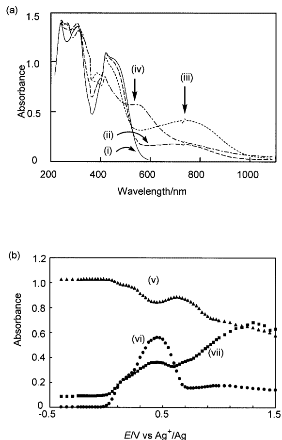
Figure 6. (a) Changes of absorption spectra of 4 (0.05 mM) in acetonitrile solution of 0.1 M \text{Et}_4\text{NBF}_4 at (i) -0.4 V, (ii) -0.1 V, (iii) 0.3 V, and (iv) 1.0 V (vs \text{Ag}^+/\text{Ag} ); (b) relative intensity changes of absorption spectra of 4 induced by oxidation potentials (v) at 440 nm, (vi) at 550 nm, and (vii) at 770 nm
