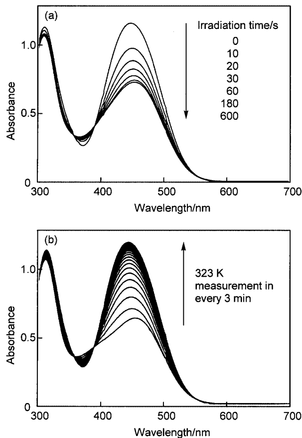
Figure 3. Change of the absorption spectrum of 4 caused by (a) photoisomerization with irradiation at 420 nm at 25 °C in toluene, and (b) thermal isomerization of the photostationary state at 50 °C in toluene
