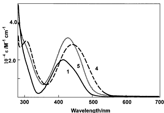
Figure 2. Absorption spectra of 1 ( 2.5 \times 10^{-5} M in \text{CHCl}_3 , solid line), 4 ( 2.5 \times 10^{-5} M in toluene, dashed line), and 5 ( 2.5 \times 10^{-5} M in toluene, dotted line) at 25 °C; wavelength at maximum absorbance and absorption coefficients are determined as: \lambda_{\text{max}} = 413 nm and \epsilon = 19900 \text{ M}^{-1}\cdot\text{cm}^{-1} ( 1 ); \lambda_{\text{max}} = 442 nm and \epsilon = 28000 \text{ M}^{-1}\cdot\text{cm}^{-1} ( 4 ); \lambda_{\text{max}} = 426 nm and \epsilon = 31500 \text{ M}^{-1}\cdot\text{cm}^{-1} ( 5 )
