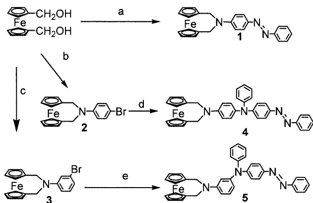
Scheme 1. (a) 4-phenylazoaniline (1 equiv.), [\text{RuCl}_2(\text{PPh}_3)_3] (5 mol %), 180 °C, NMP; (b) 4-bromoaniline (1 equiv.), [\text{RuCl}_2(\text{PPh}_3)_3] (5 mol %), 180 °C, NMP; (c) 3-bromoaniline (1 equiv.), [\text{RuCl}_2(\text{PPh}_3)_3] (5 mol %), 180 °C, NMP; (d) 4-phenylazo-diphenylamine (1 equiv.), [\text{Pd}_2(\text{dba})_3] (1.3 mol %), \text{NaOtBu} (1.5 equiv.), \text{P}(t\text{Bu})_3 (7.5 mol %), 100 °C, toluene
