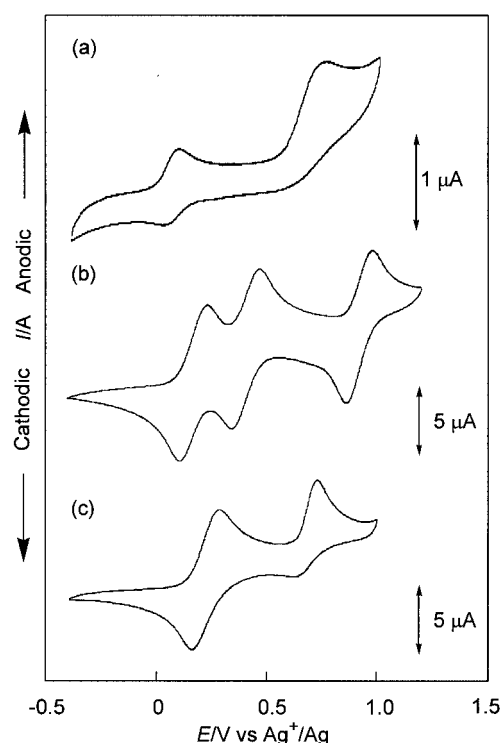
Figure 5. Cyclic voltammograms of (a) 1 (1.0 mM) in \text{CH}_2\text{Cl}_2 containing 0.10 M \text{Et}_4\text{NBF}_4 ( E_{1/2} = 0.05 V and E_{\text{pa}} = 0.75 V), (b) 4 (1.0 mM) in \text{CH}_2\text{Cl}_2 containing 0.10 M \text{Et}_4\text{NBF}_4 ( E_{1/2} = 0.17 V, 0.41 V, and 0.92 V), and (c) 5 (1.0 mM) in \text{CH}_2\text{Cl}_2 containing 0.10 M n\text{Bu}_4\text{NPF}_6 ( E_{1/2} = 0.22 V and E_{\text{pa}} = 0.73 V); sweep rate: 0.10 V \text{s}^{-1} ; measurement was carried out at 25^\circ\text{C}
